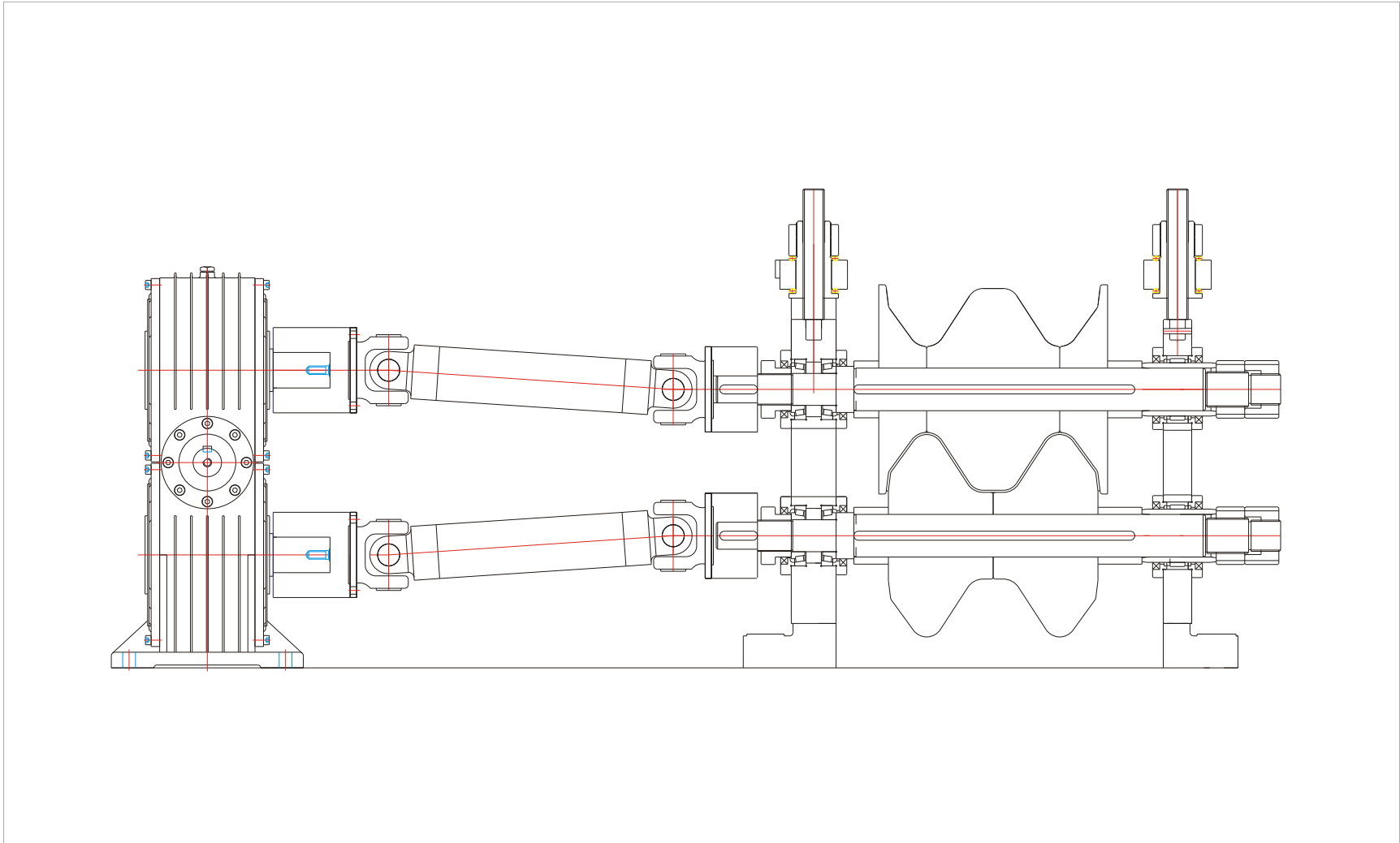
Worm Gear Box Driven Universal Shaft
