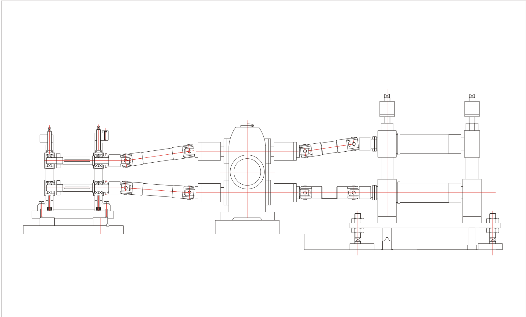
Duplex Design Roll Former
